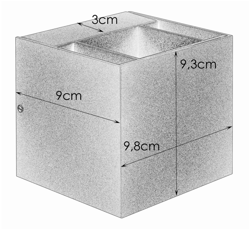
BACK SIDE INSTALL DIMENSIONS
